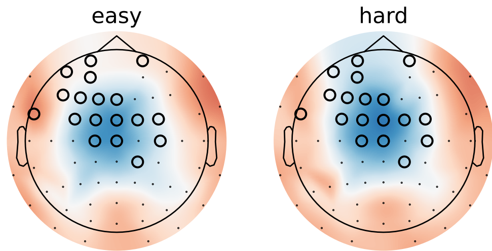
Difficulty effect ( p = 0.015 ) 0.676–1.124 s
