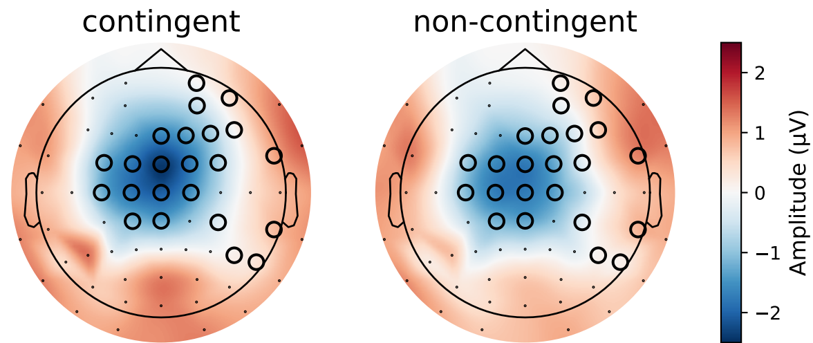
Contingency effect ( p = 0.002 ) 0.752–1.200 s
