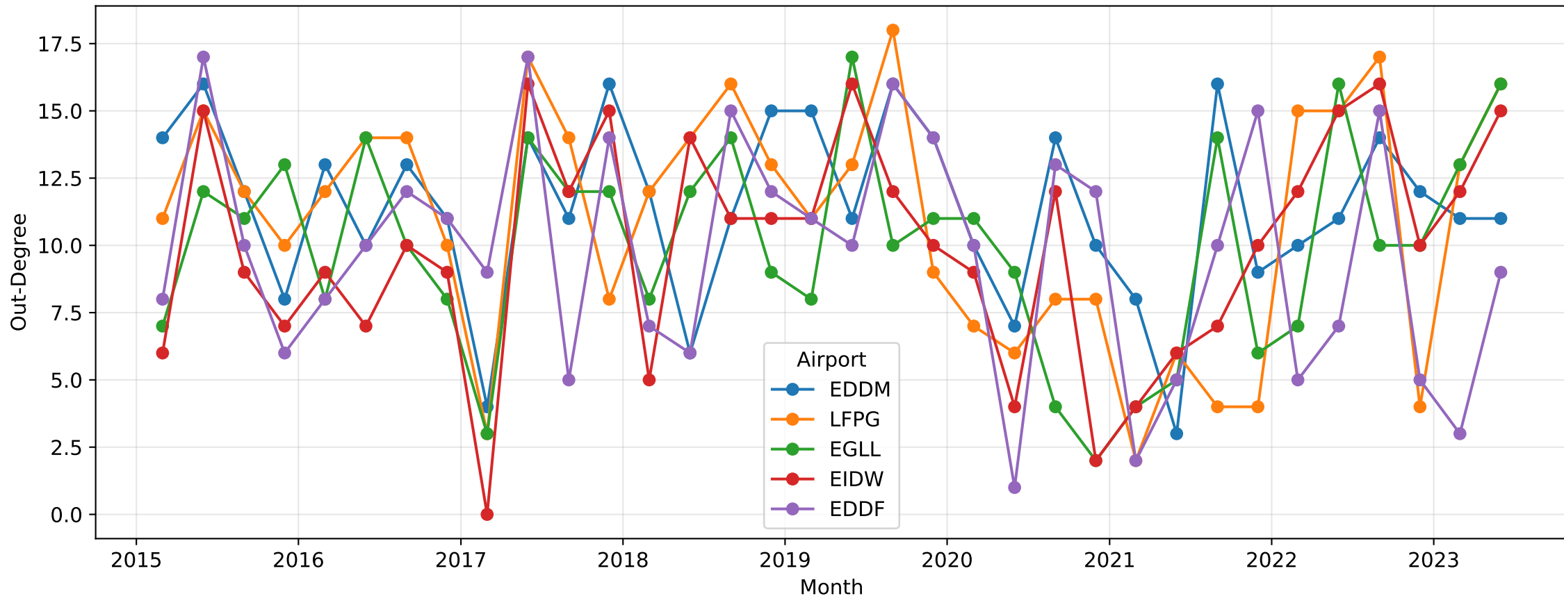
Top Delay Spreaders Over Time (FULL Network, Monthly)
