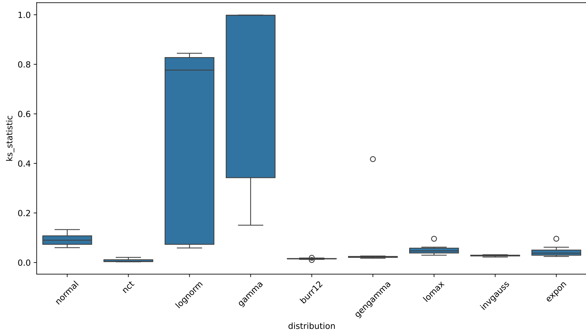
Distribution of KS Statistics by Distribution Type
