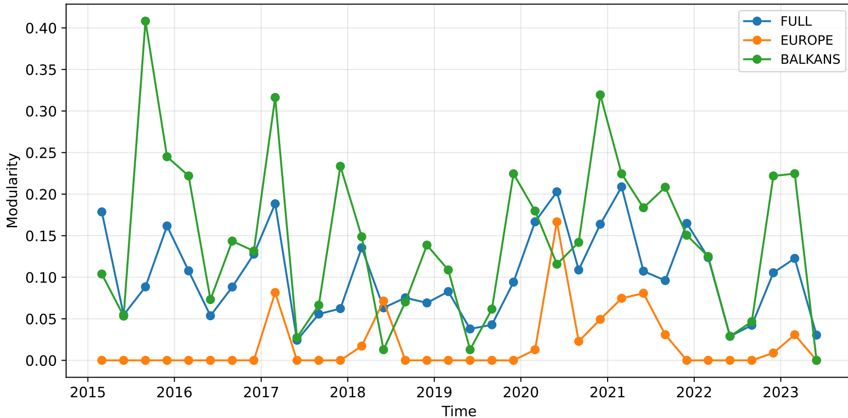
Modularity Over Time
