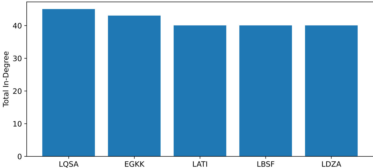
Top Delay Receivers in 2018 (In-Degree)
