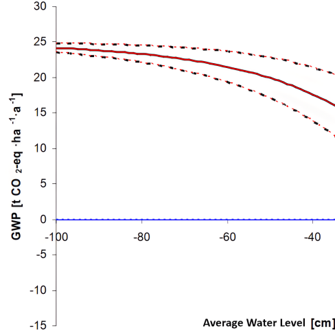
Figure A.6: Greenhouse gas emissions and water-table depth
