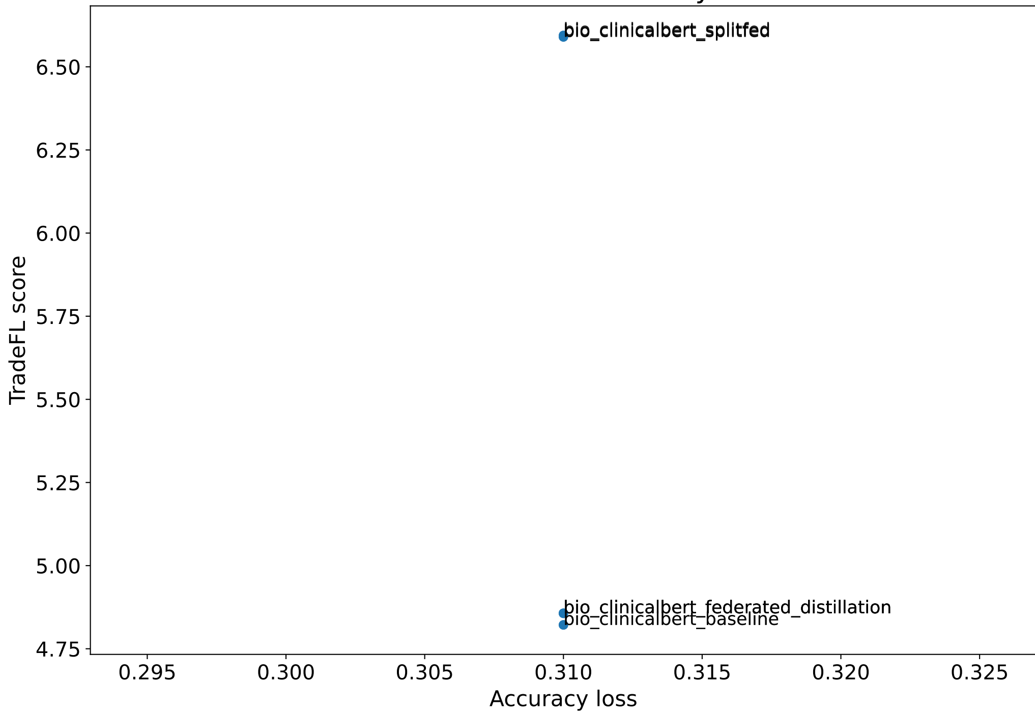
TradeFL score vs accuracy loss
