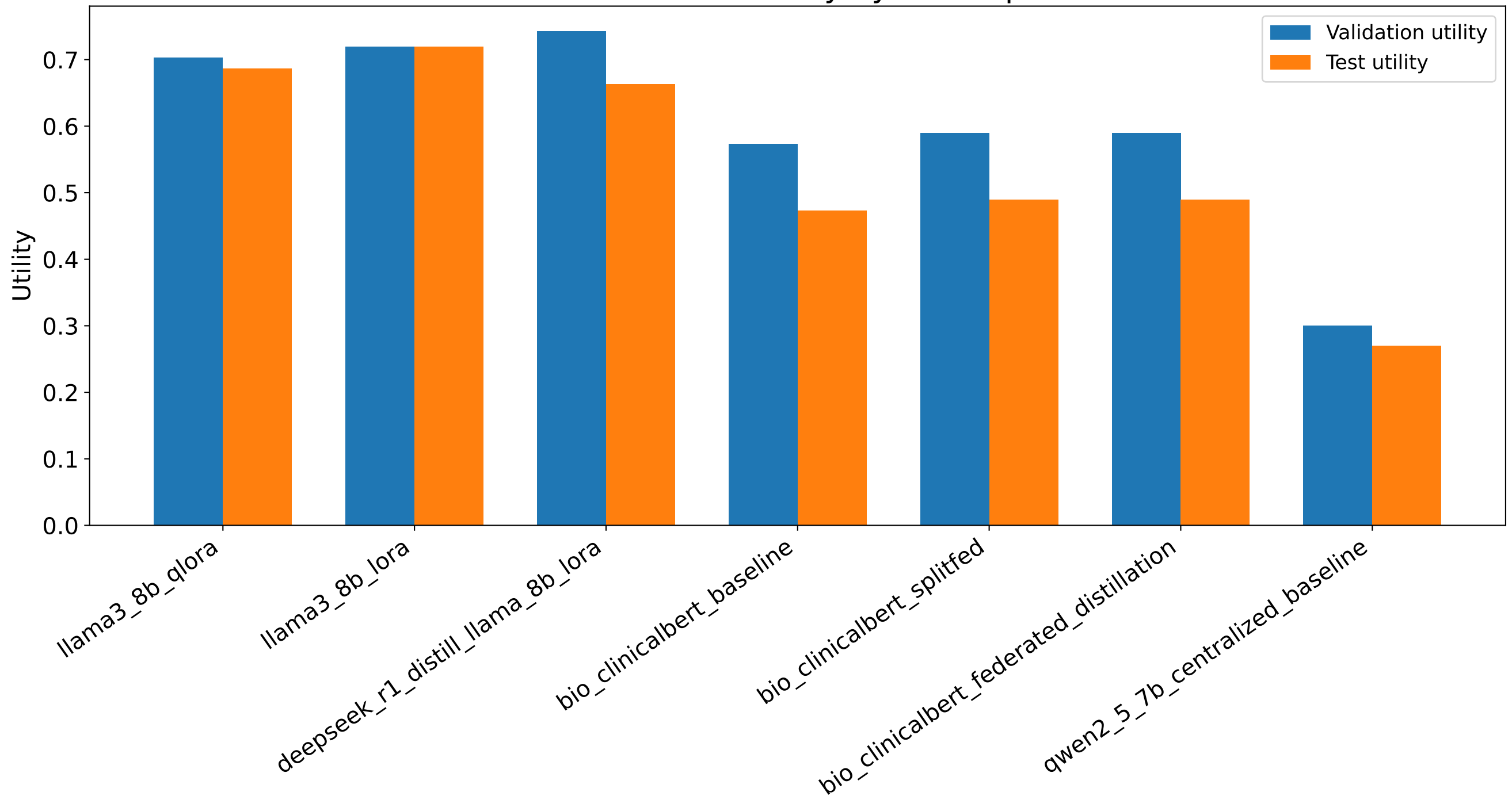
Validation/test utility by model plan
