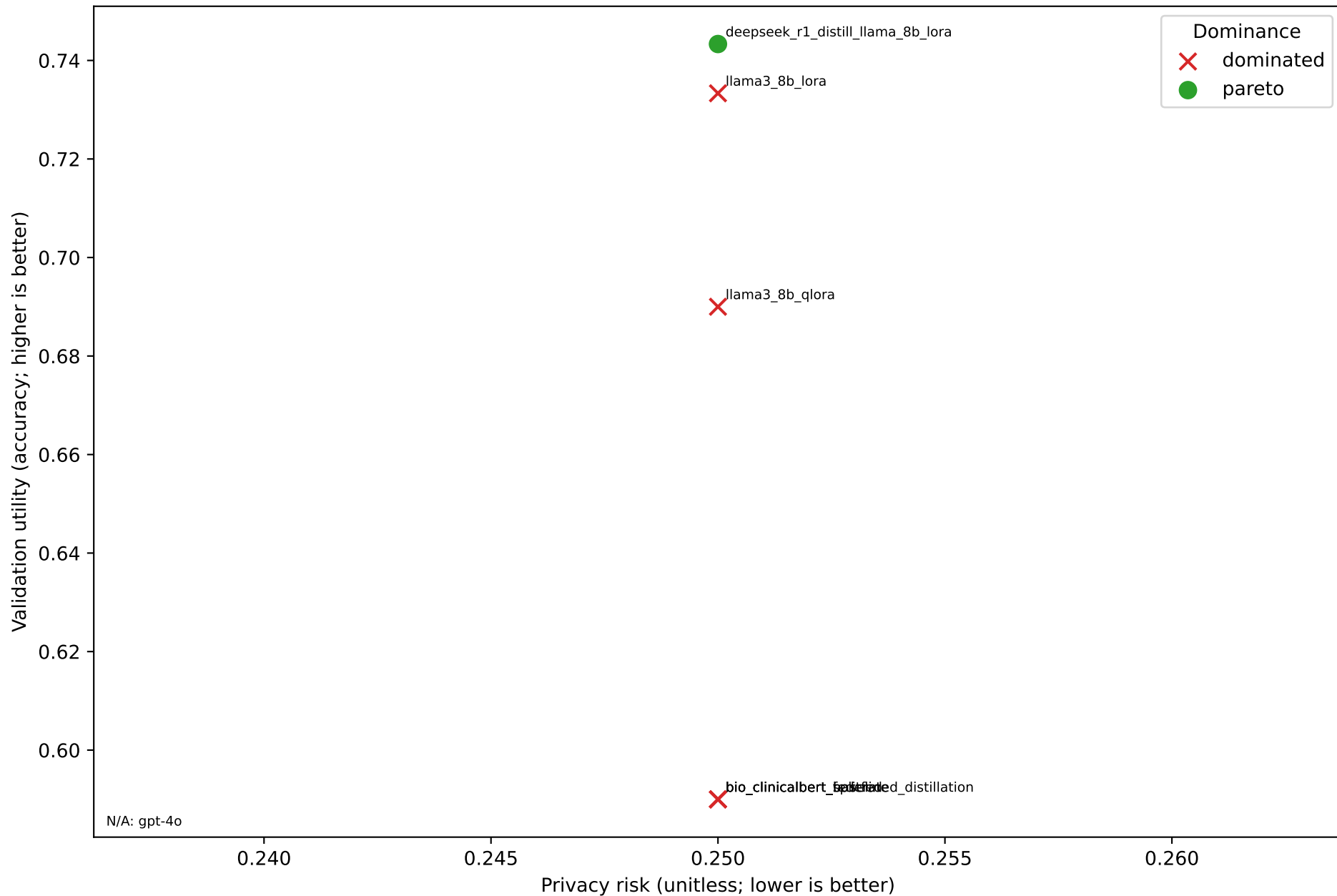
Pareto view: privacy accuracy
