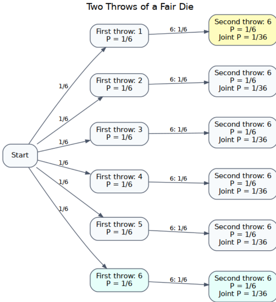
Figure 2: Tree
