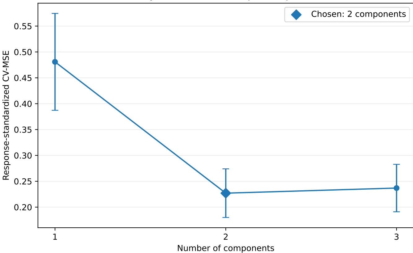
Synthetic Pi-PLS component path
