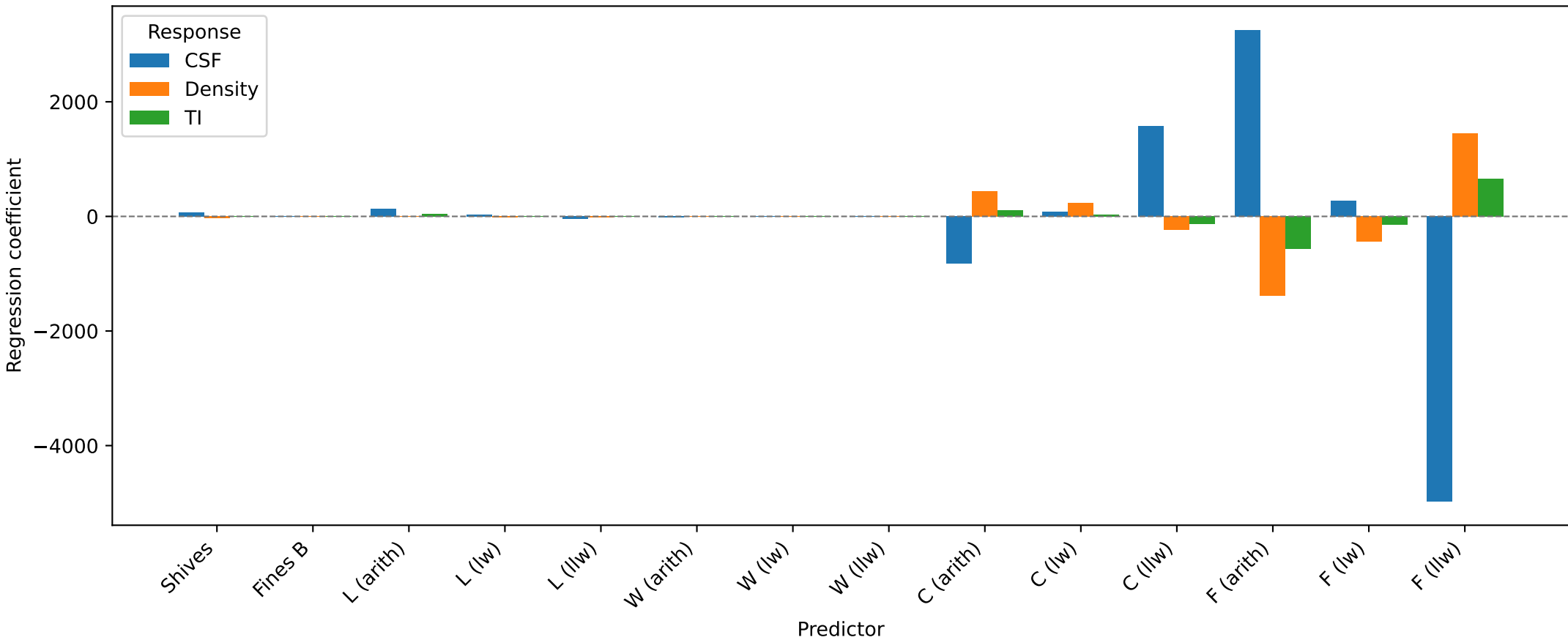
Pulp Pi-PLS coefficients
