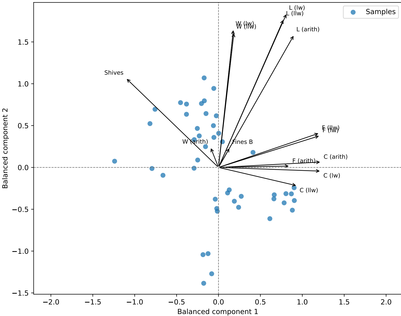
Pulp Pi-PLS score-loading biplot
