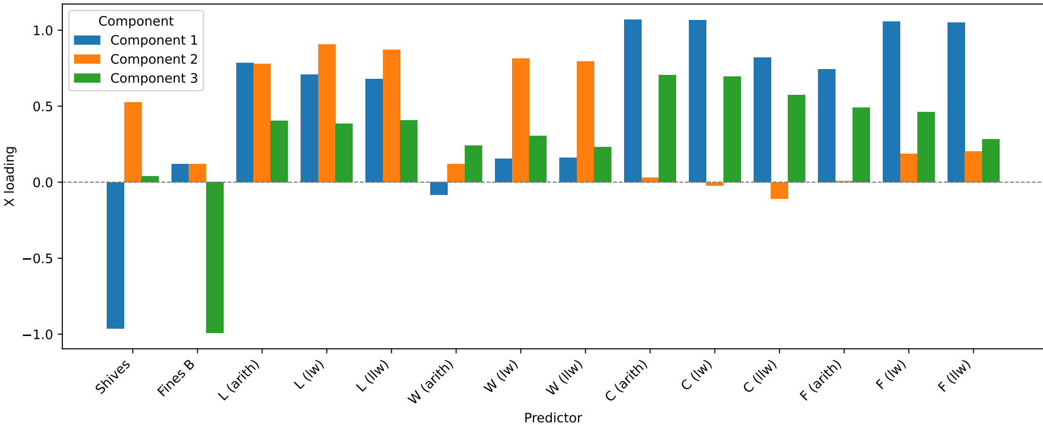
Pulp Pi-PLS X loadings
