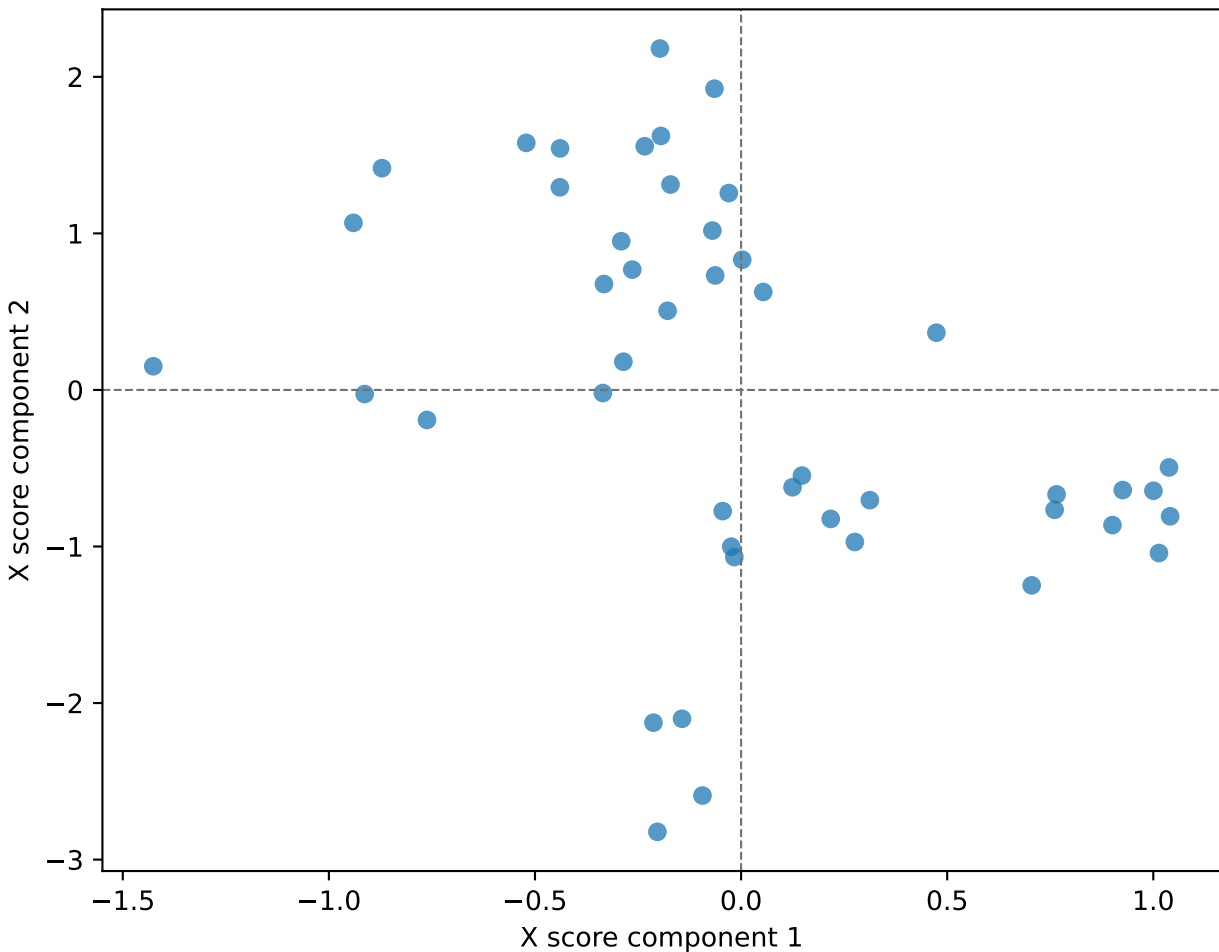
Pulp Pi-PLS X scores
