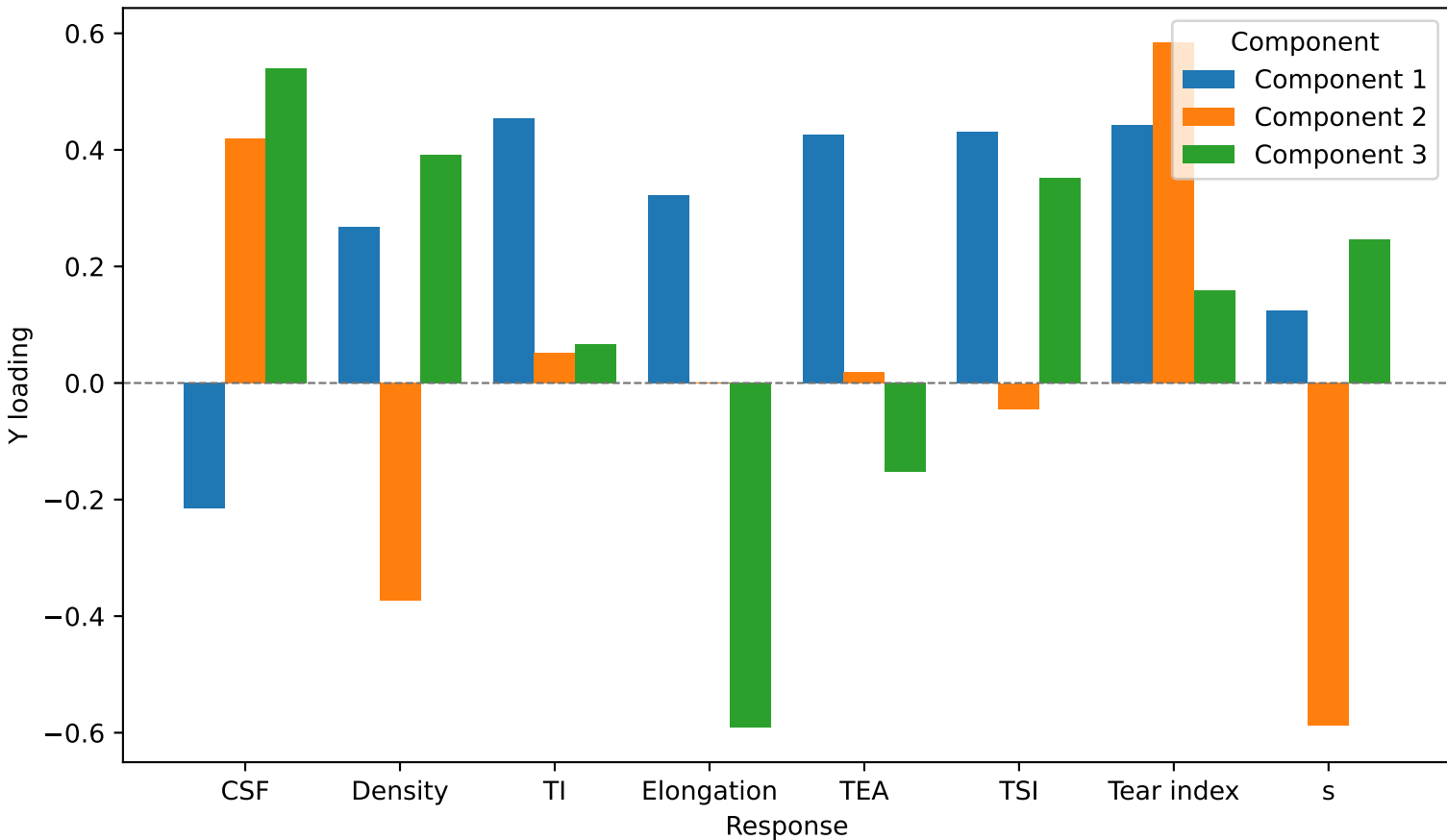
Pulp Pi-PLS Y loadings
