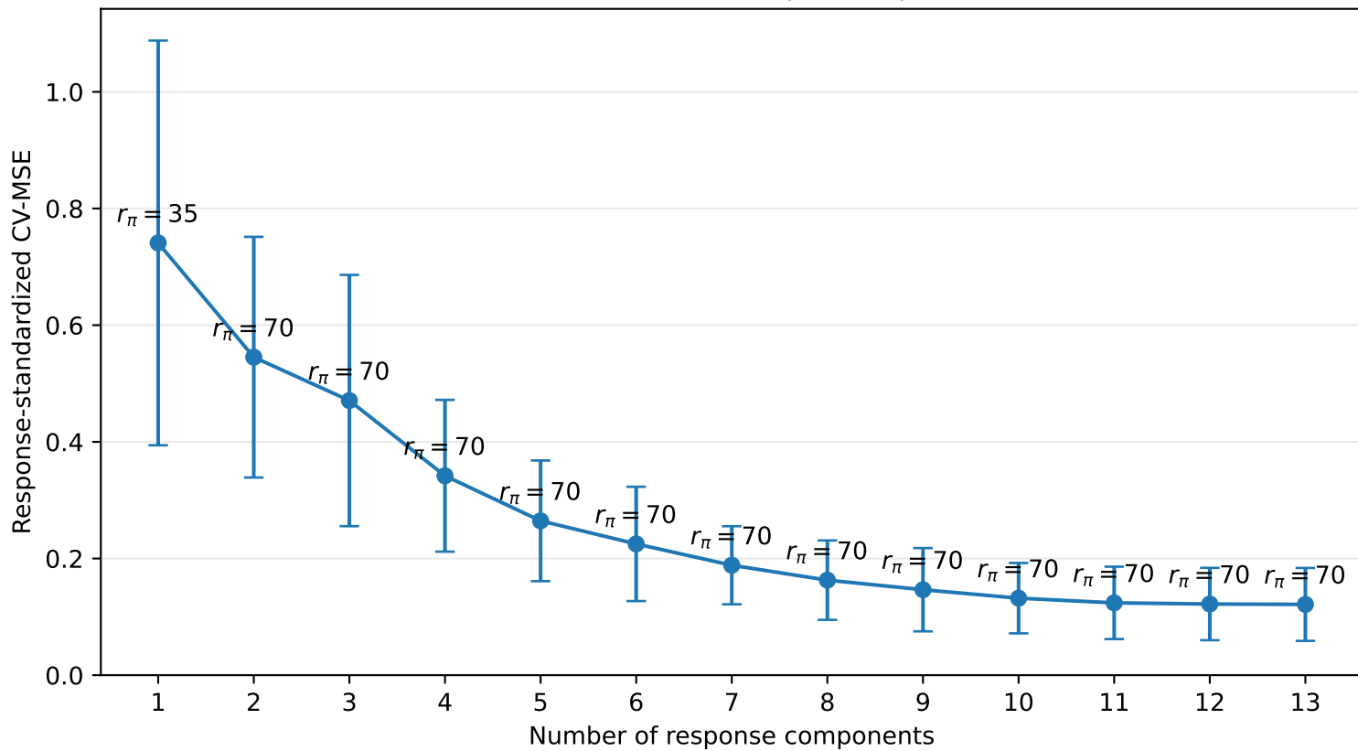
Tobacco Pi-PLS component path
