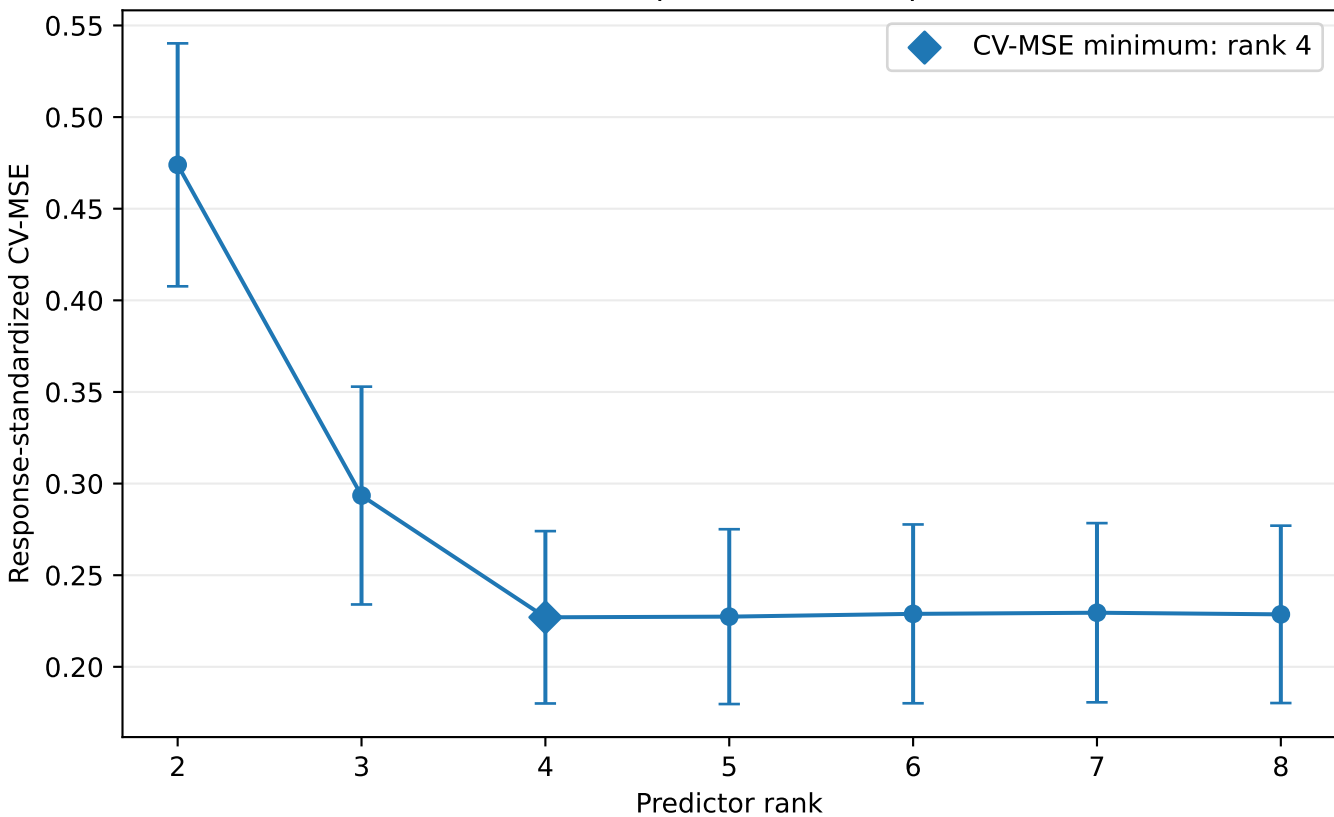
Predictor-rank profile at 2 components
