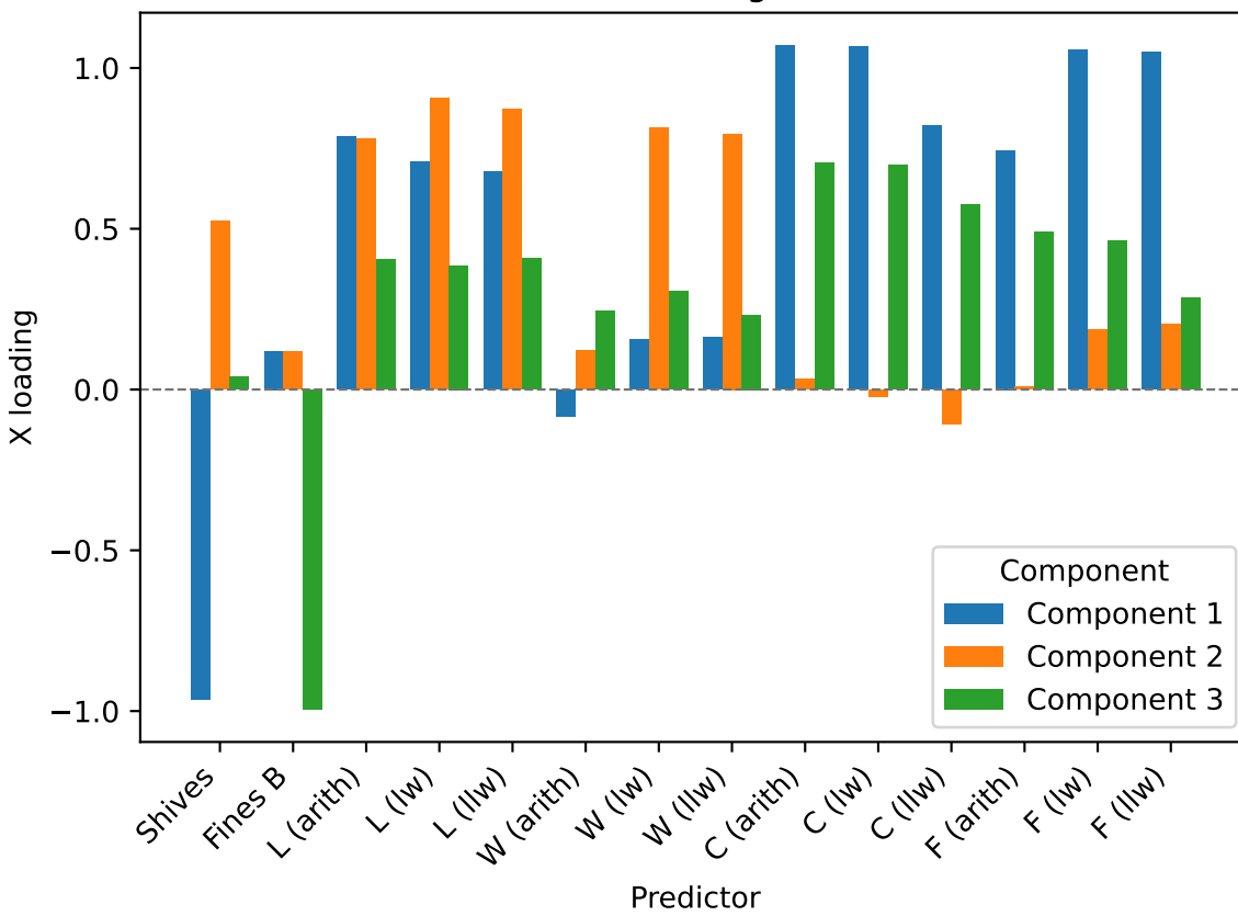
X loadings
