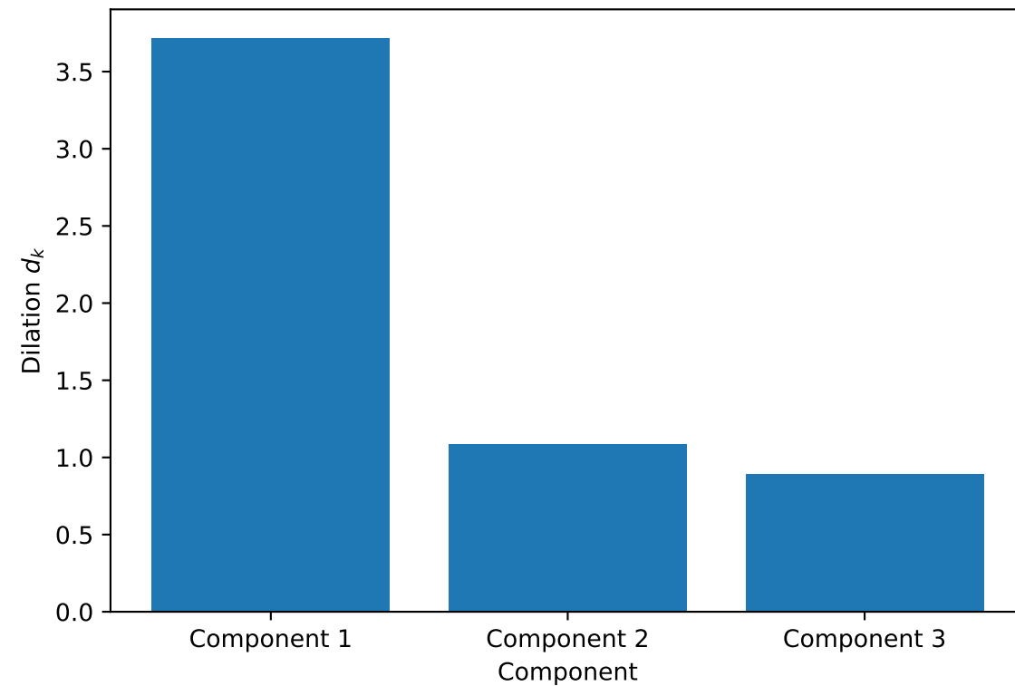
Pi-PLS dilation
