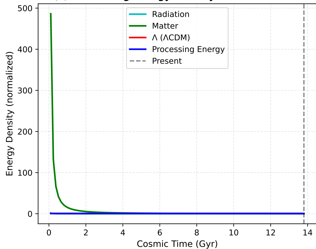
(c) Processing Energy Density of the Universe
