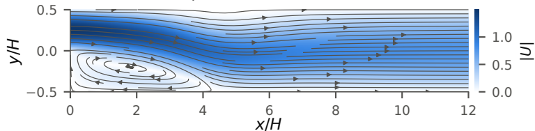
(c) pitzDaily, 10 m/s, k-\varepsilon
