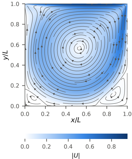
(a) Lid-driven cavity, Re = 1000
