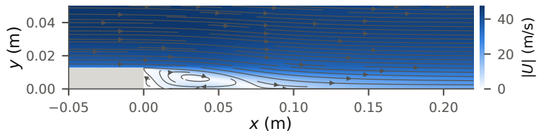
(d) Pawar--Maulik step, 44.2 m/s, k-\omega SST (near-step region)
