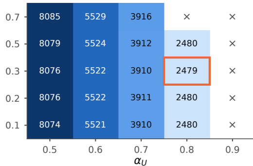
(b) Laminar step Re = 400 (SIMPLE)
