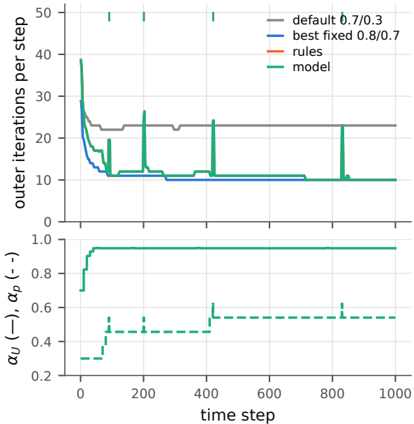
(a) pitzDaily, 20 m/s, \Delta t = 0.1 ms (held out)
