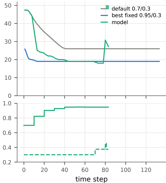
(b) 3D cavity, Re = 400 , \Delta t = 0.3 (held out): crash
