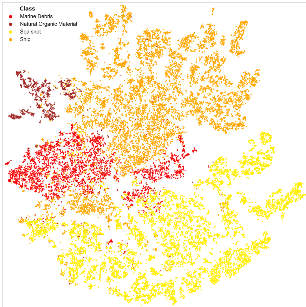
Fig. 7. T-SNE Analysis on MADOS dataset using Spectral Angle Mapping for Marine Debris, Ship, Natural Organic Material and Sea snot.
