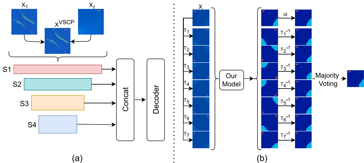
Fig. 3. Simplified overview of MariNeXt, which consists of two main parts: a) During the training process, the input batch of images is augmented using the VSCP module combining the samples, which are then passed as new input. Then MariNeXt exploits the S1 (1 st -Stage Higher Resolution Features) to produce fine-grained predictions. b) During testing, the Test-Time Augmentation (TTA) strategy is employed to produce several augmented views of the input image and aggregate the predictions by major voting, producing refined predictions.
