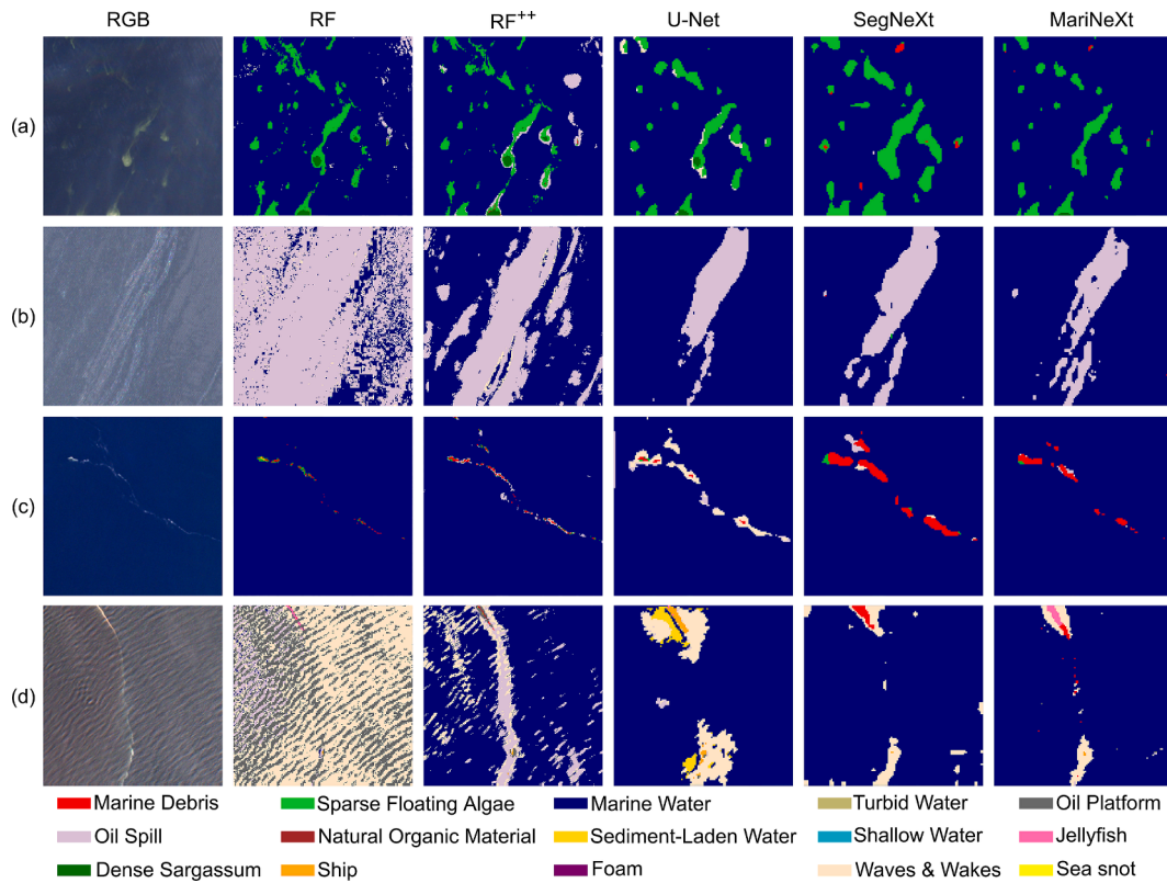
Fig. 5. Prediction maps extracted by the applied baselines and MariNeXt. The RGB images show: a) Dense & sparse Sargassum, Marine Water and haze/thin clouds, b) Oil Spill and Marine Water, c) Marine Debris and Marine Water, and d) Jellyfish and rough sea state. The RGB images were stretched for illustration purposes. For more classification results, the reader is referred to Supplementary Figure S1.
