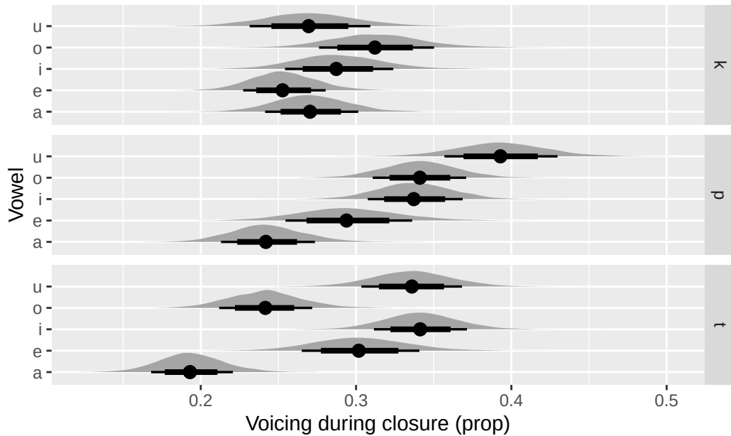
Figure 5: Expected predictions of voicing proportion by vowel and consonant from voi_prop_bm .
