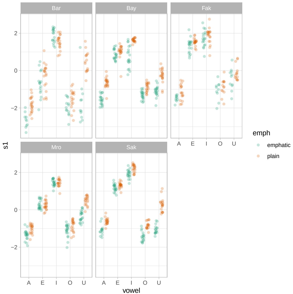
Figure 17 PC1 scores of emphatic and plain consonants by speaker and vowel.
