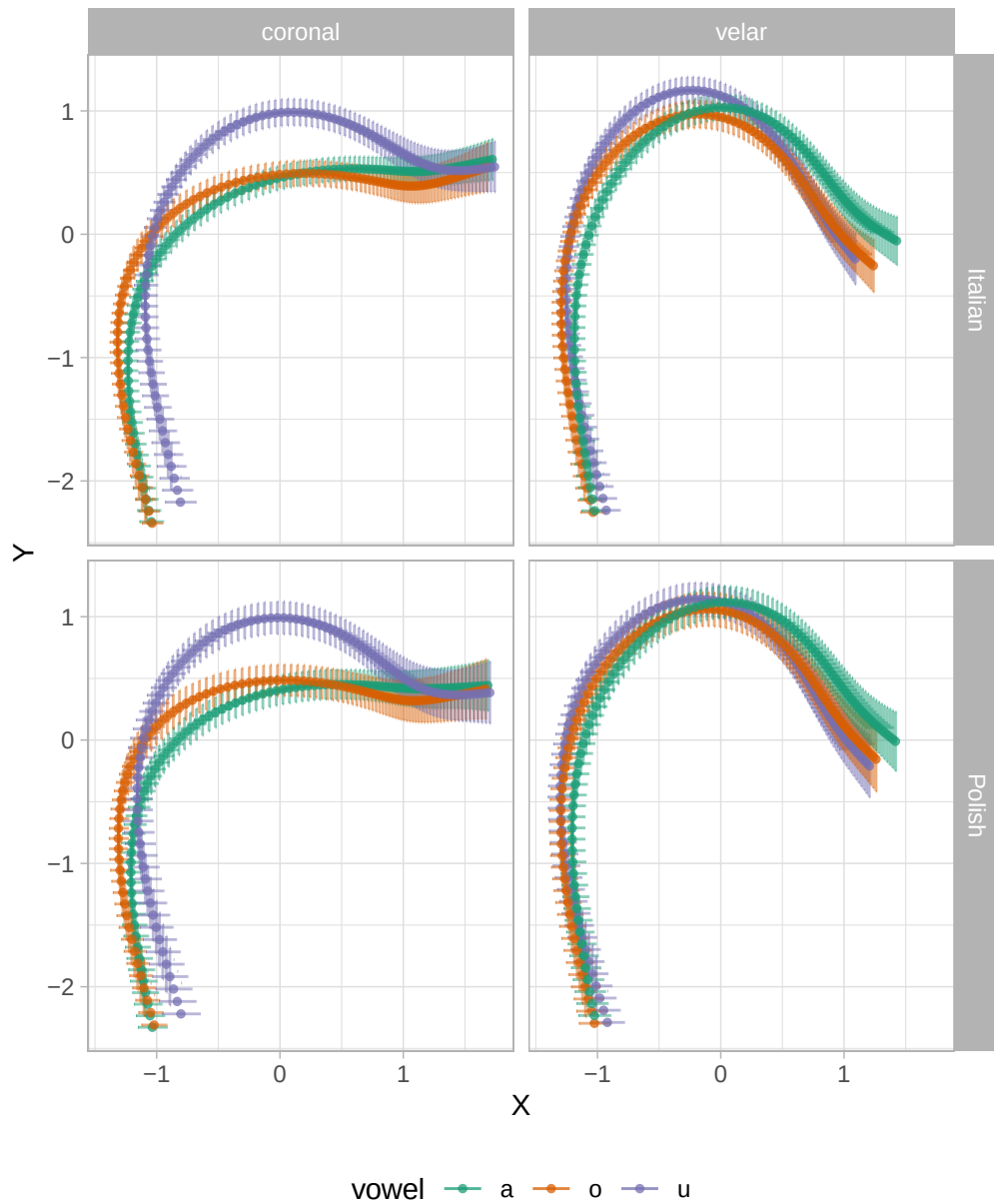
Predicted tongue contours based on a multivariate GAM, with 95% Confidence Intervals.
