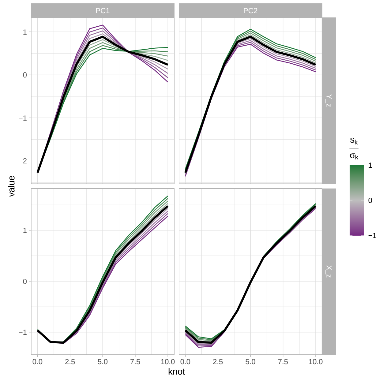
Figure 12 Predicted curves along knot number for X and Y coordinates, as obtained from an MFPCA.
