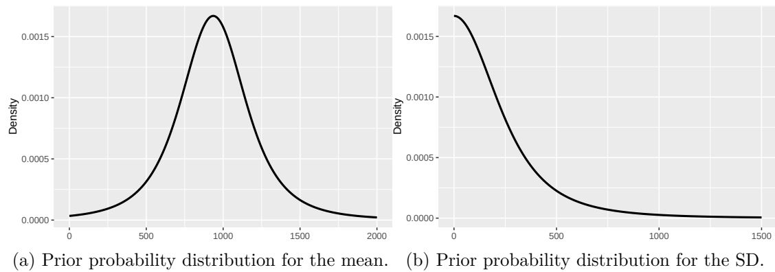
Figure 22.1: Default brms priors for this chapter's model and data.
