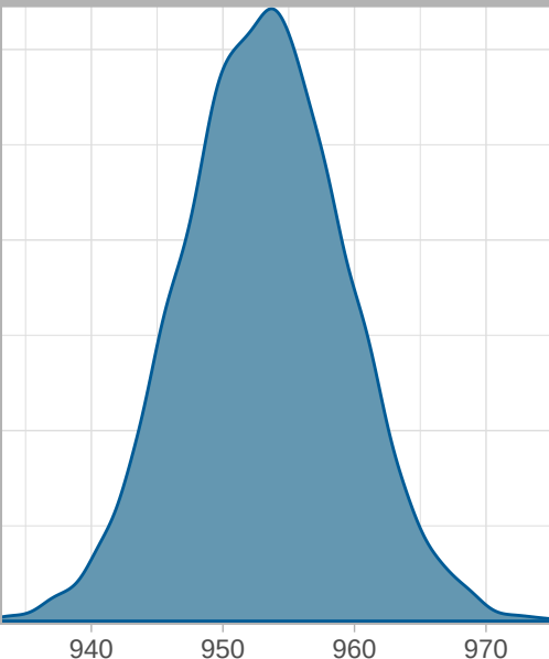
b_Intercept
