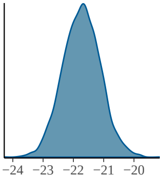
b_speech_rate
