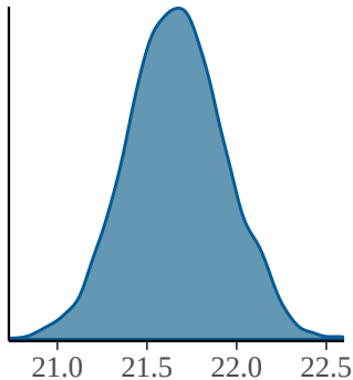
sigma
