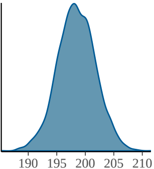
b_Intercept
