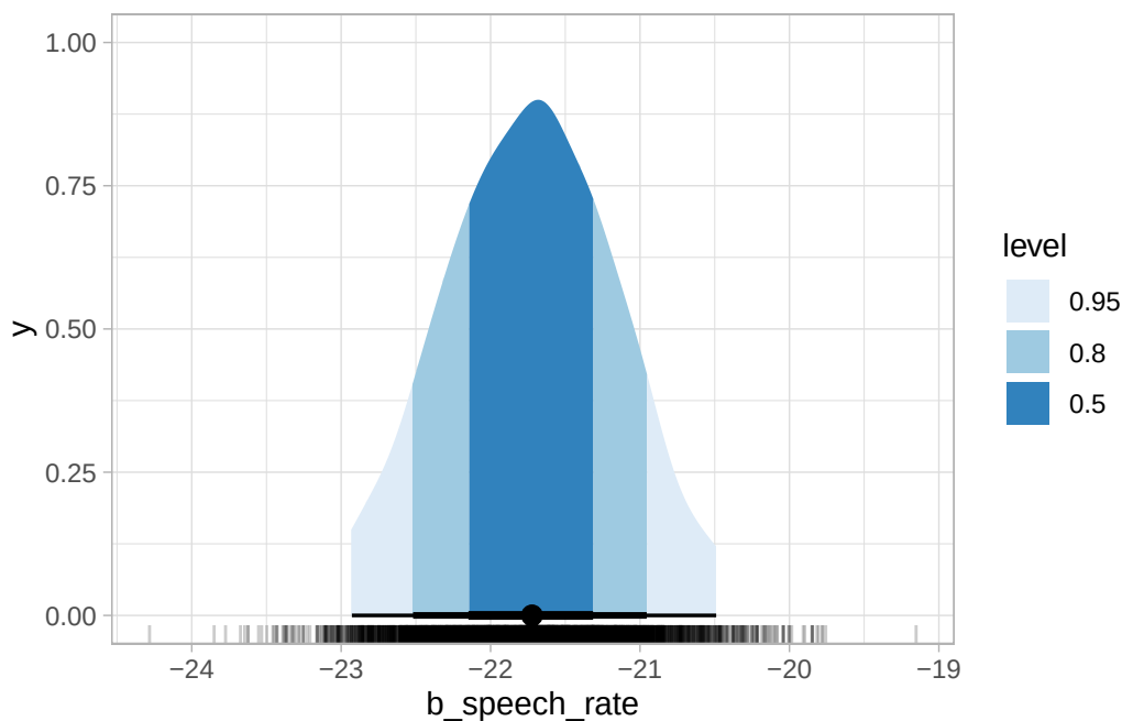
Figure 25.4: Posterior probability distribution of b_speech_rate with credible intervals.
