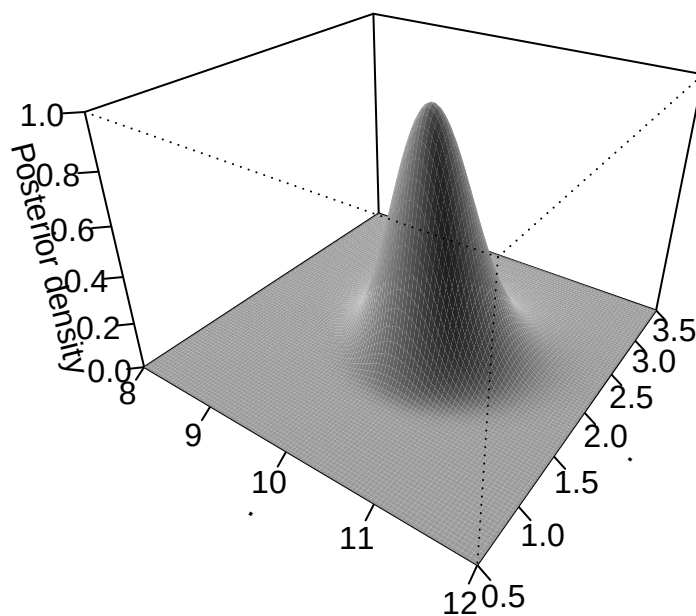
Figure 25.1: 3D representation of the joint posterior probability distribution of \mu and \sigma from a Bayesian Gaussian model.
