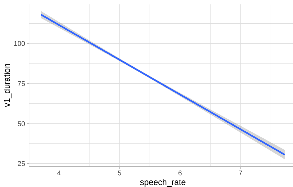
Figure 25.5: Conditional mean (expected value) of vowel duration based on speech rate from a regression model.
