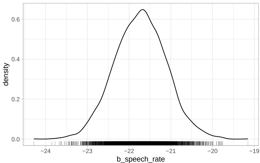
Figure 25.3: Posterior probability distribution of b_speech_rate .
