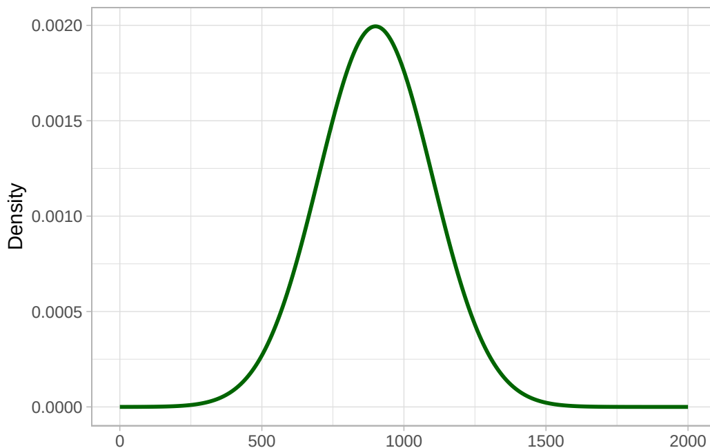
Figure 21.2: The prior for \mu .
