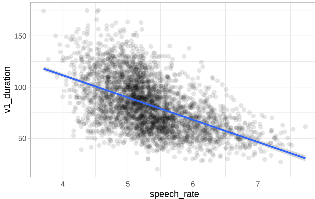
Figure 25.6: Conditional mean (expected value) of vowel duration based on speech rate from a regression model (repr.).
