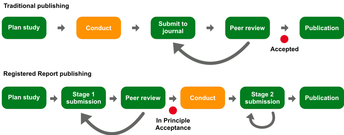
Figure 33.2: A comparison of traditional publishing vs registered reports.
