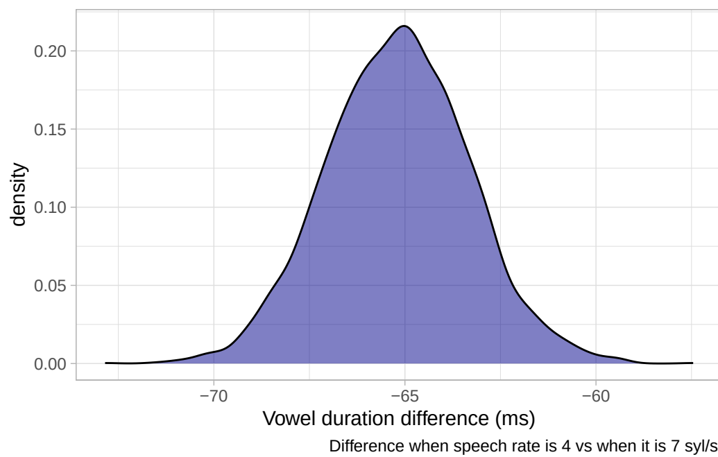
Figure 25.7: Posterior distribution of the difference in vowel duration at 4 vs 7 syl/s.
