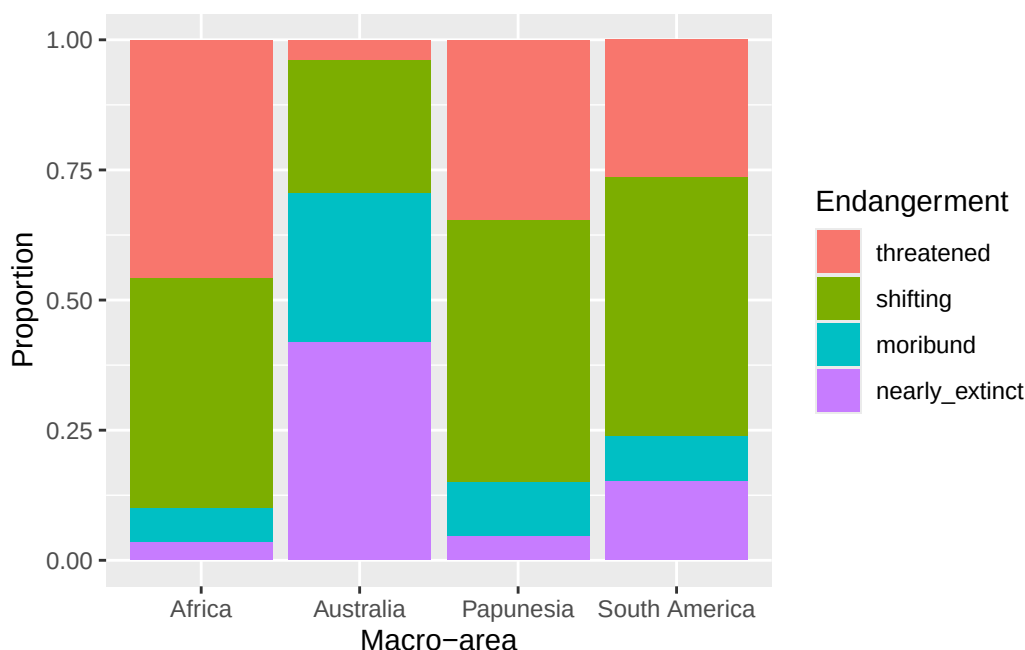
Figure 17.4: Proportion of languages by macro-area and endangerment status.
