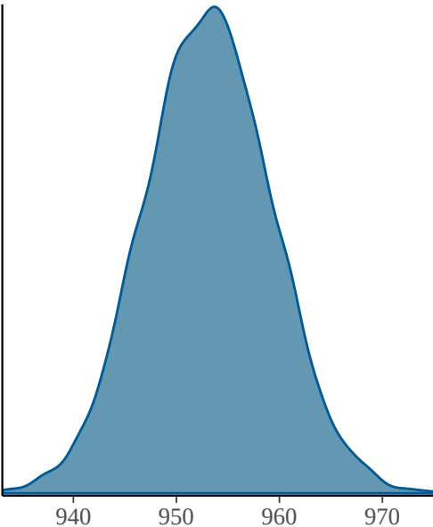
b_Intercept
