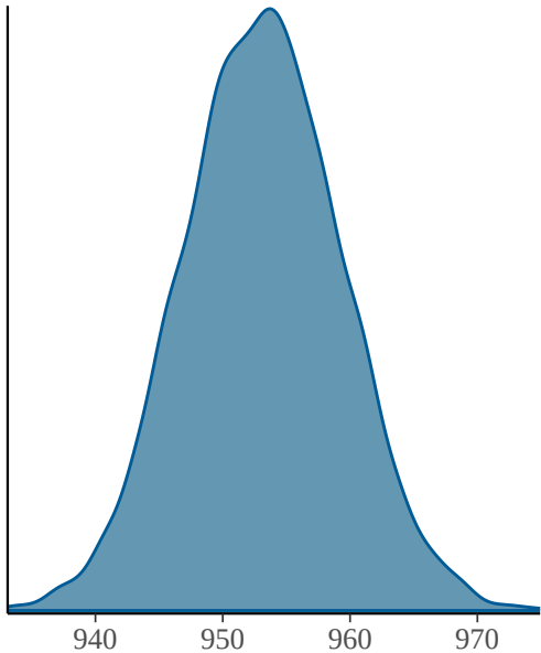
b_Intercept
