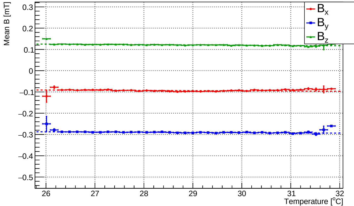
Mean magnetic field vs temperature
