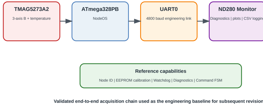
Figure 5.1: RV-01 – Reference Single-Sensor Platform. The reference acquisition chain couples one TMAG5273A2 sensor to the ATmega328PB running NodeOS and exposes the resulting measurements and diagnostics to the ND280 Monitor through UART.
