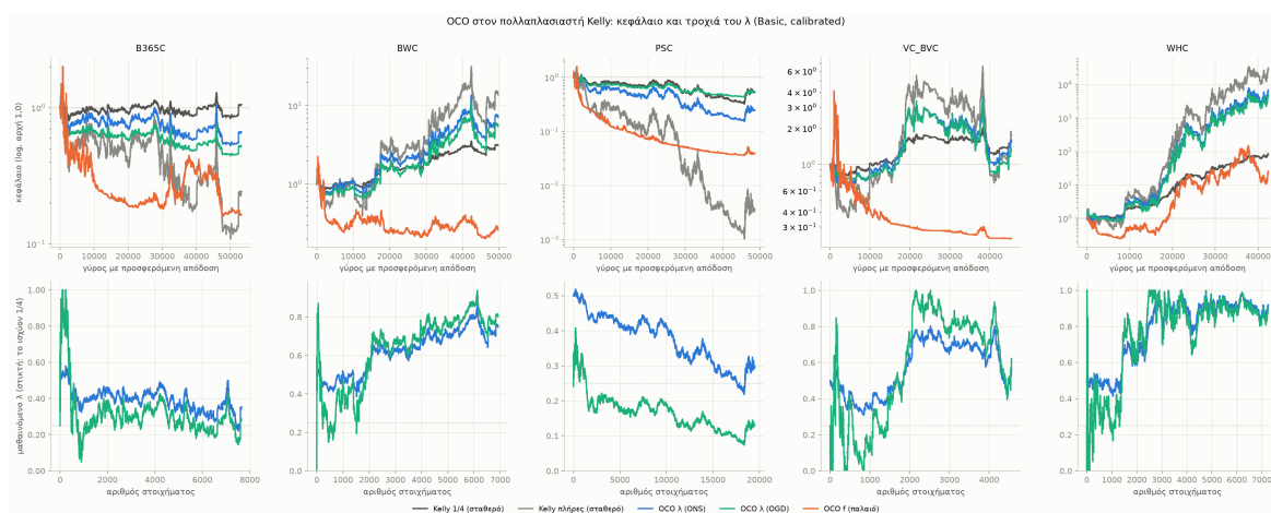
Figure 7.9: Above, the path of the bankroll; below, the trajectory of the learned \lambda with a dotted line at the \frac{1}{4} in force.
