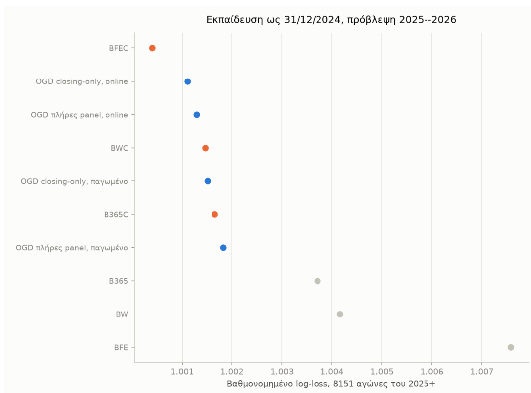
Figure 5.8: Deployment test. The opening prices sit clearly lower, while the closing prices and the variants of the mixture cluster together.
