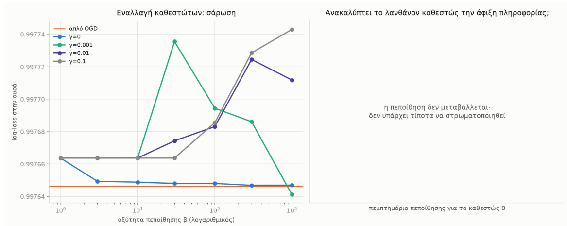
Figure 5.11: Left, the sweep of the belief sharpness. Right, the check of whether the latent regime corresponds to the measured information arrival.
