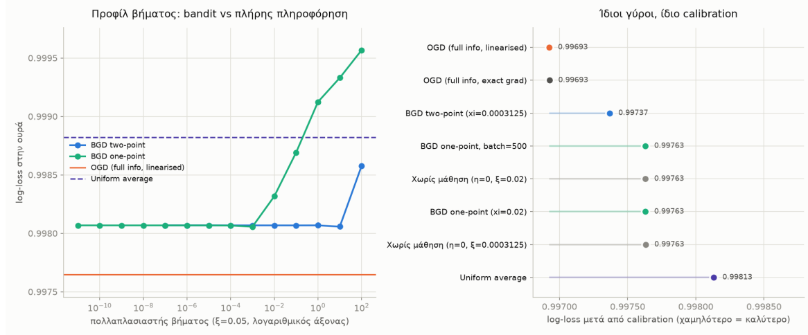
Figure 5.10: Left, the step profile on which the selection is made; right, the final comparison.
