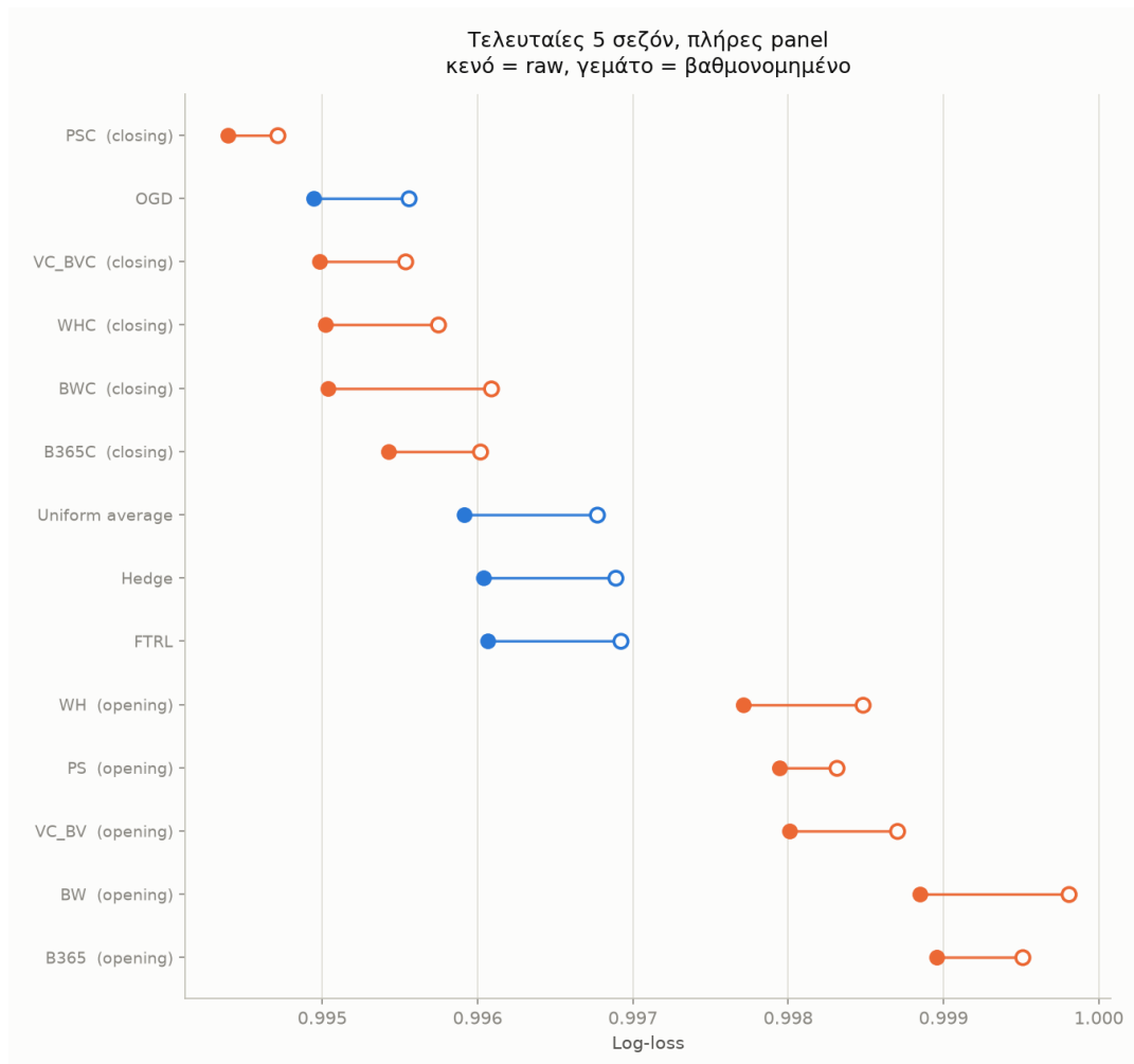
Figure 5.7: Last five seasons. The closing bookmakers now pass the coverage threshold and the comparison becomes more demanding.
