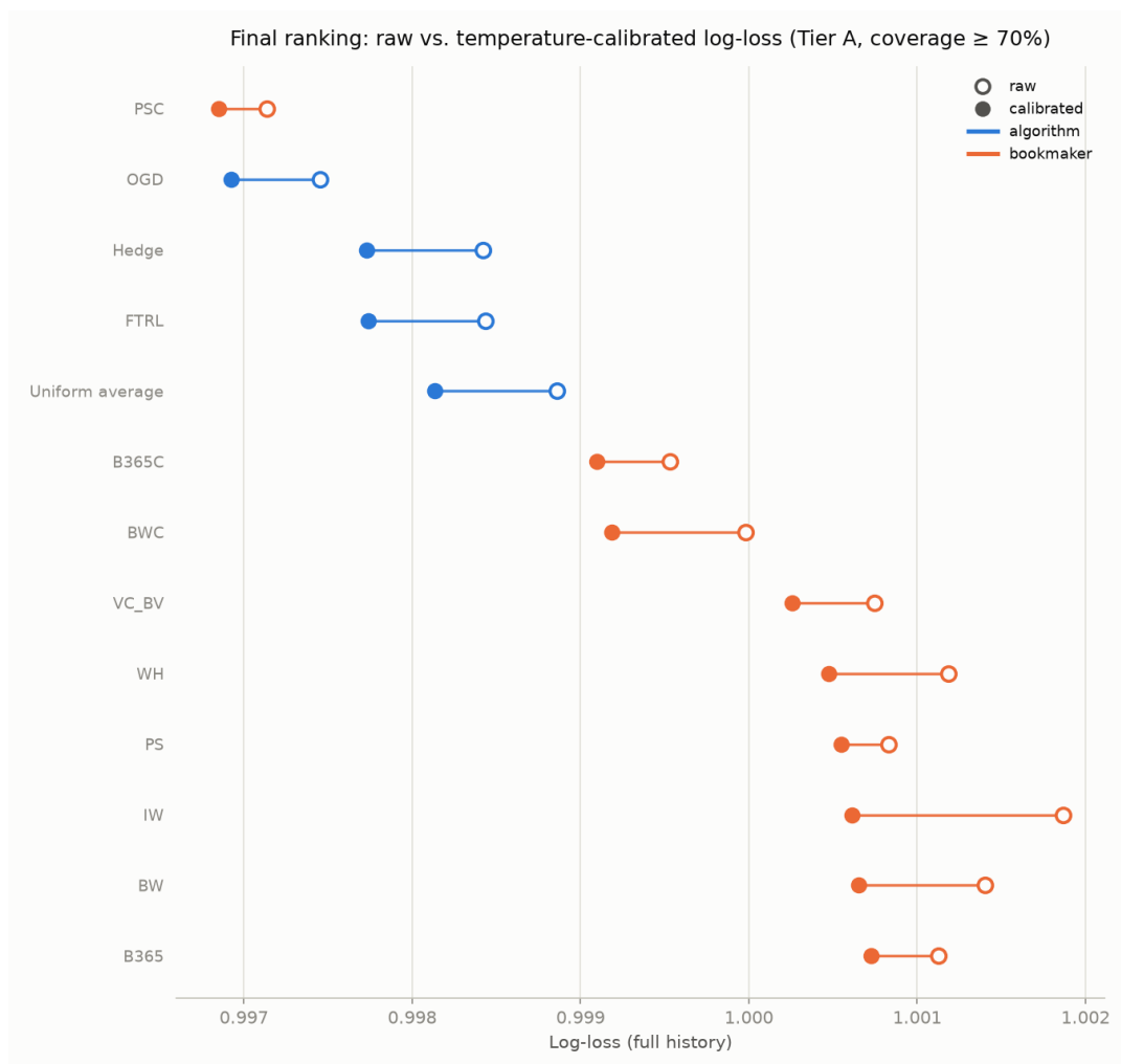
Figure 5.2: Each row: hollow circle the raw log-loss, filled the calibrated one. The choice of a dot/slope plot rather than a bar chart is deliberate, since log-loss values cluster around 1.0 with no meaningful zero and a bar chart with a truncated axis would visually exaggerate minute differences.
