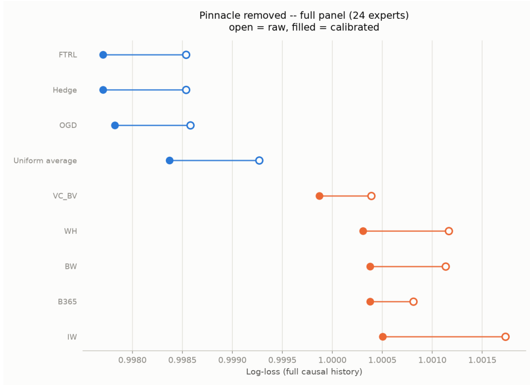
Figure 5.6: Full panel without any Pinnacle column. All four methods sit above all remaining bookmakers.
