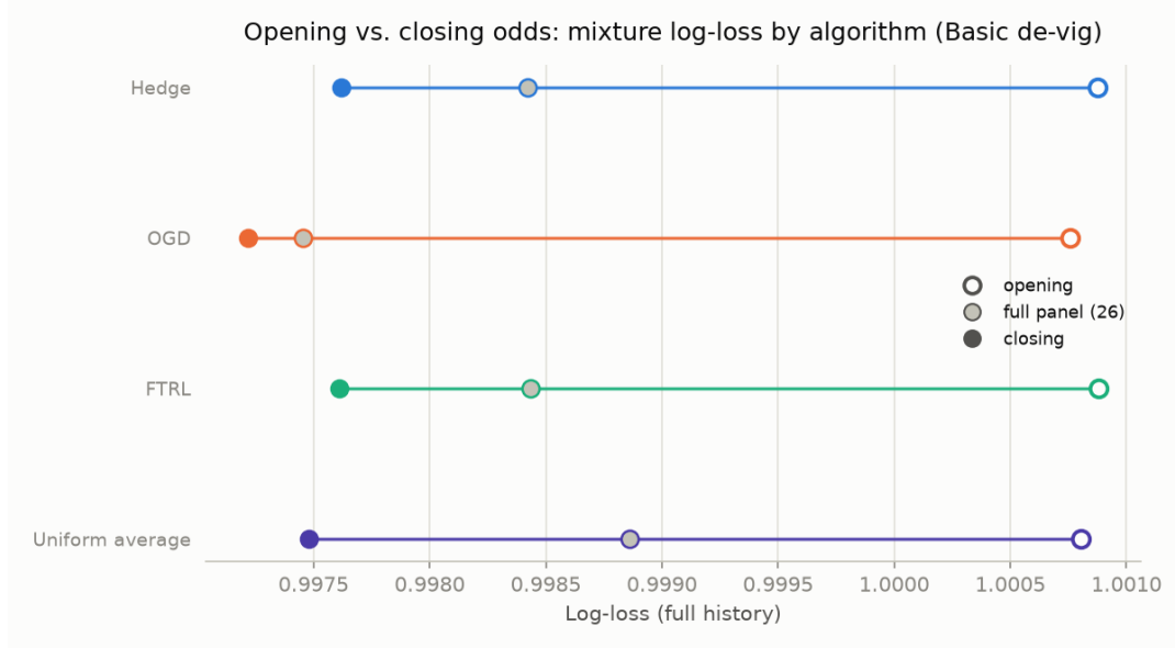
Figure 5.3: Comparison of the three panels for each algorithm. The ordering closing < all < opening holds in every case.
