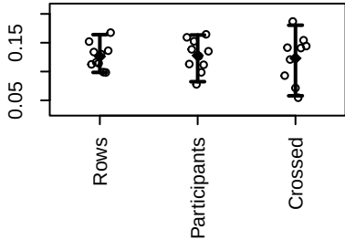
Brier score
