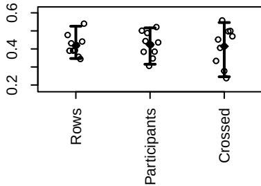
Log loss
