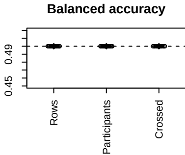
Balanced accuracy
