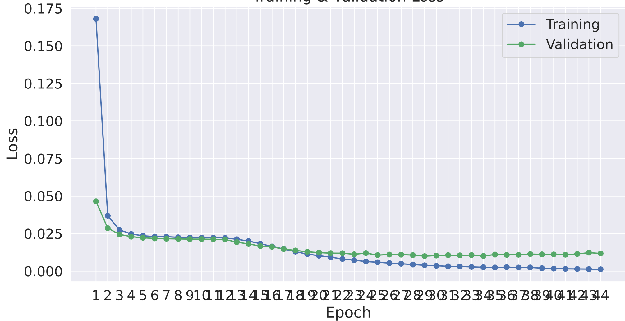
Training & Validation Loss
