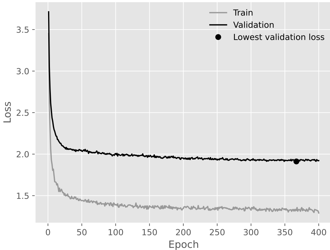
Loss: coarse annotations + RGB images
