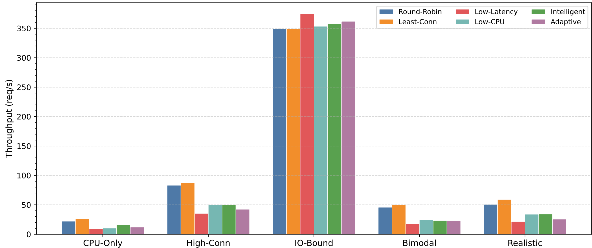
Throughput by Workload Profile and Algorithm
