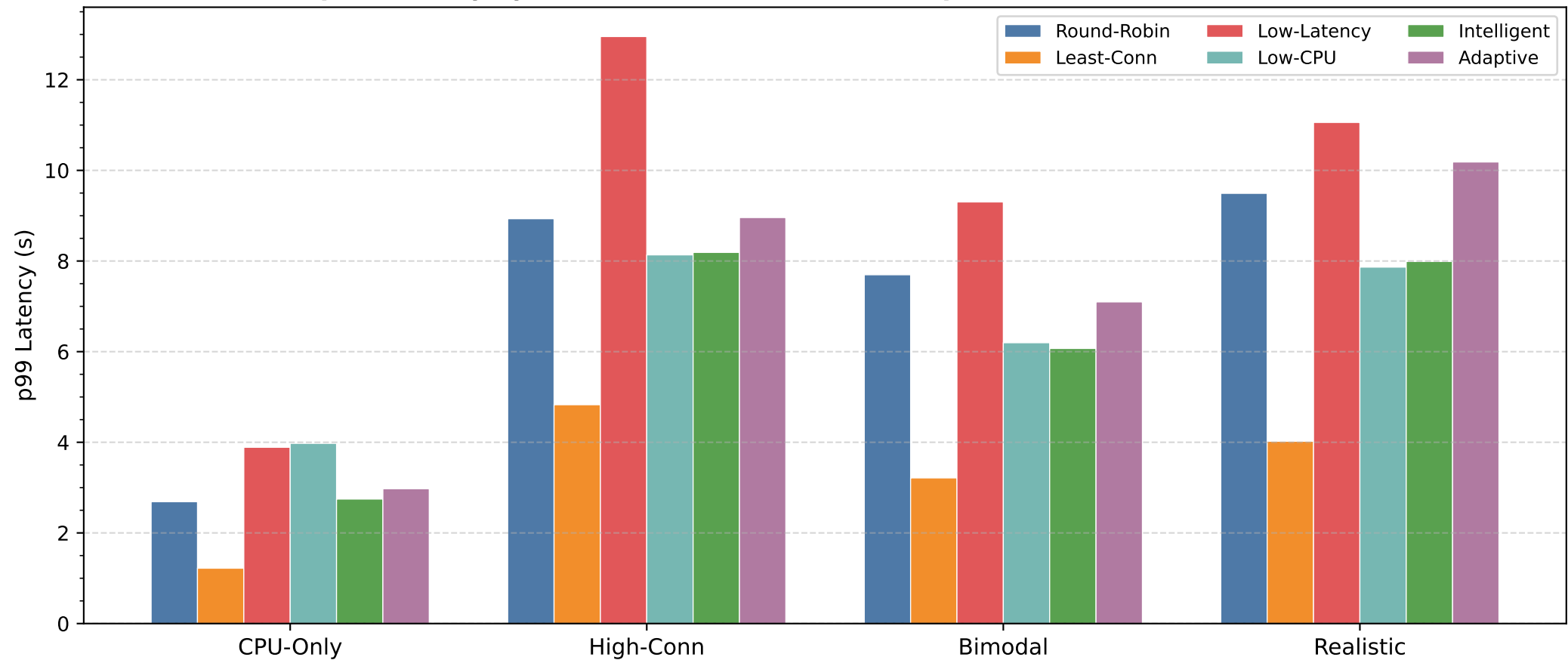
p99 Latency by Workload Profile (CPU-bound profiles, excludes IO-Bound)
