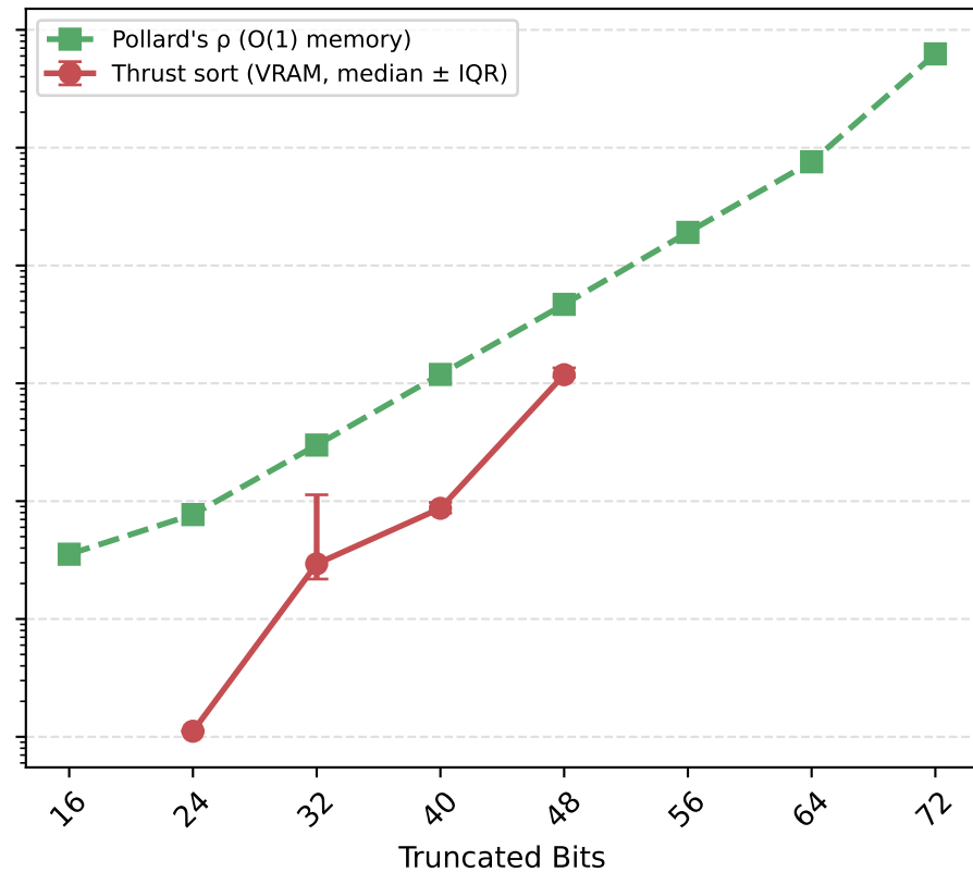
SHA-256
