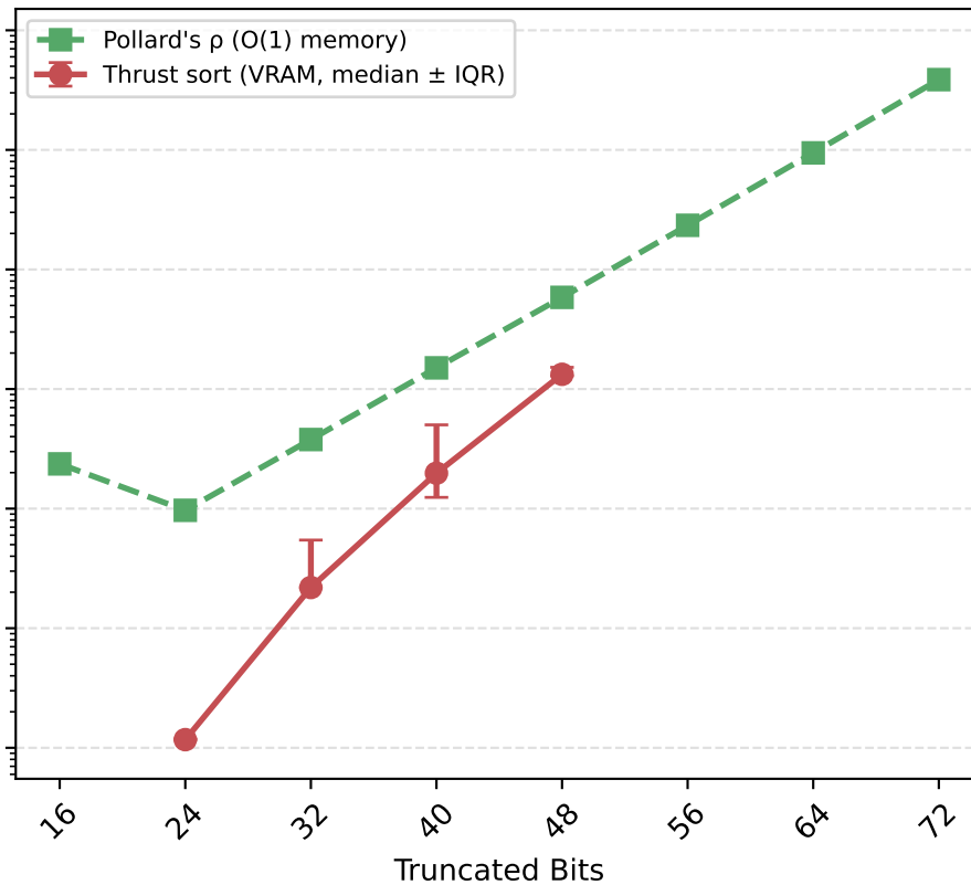
SHA-1
