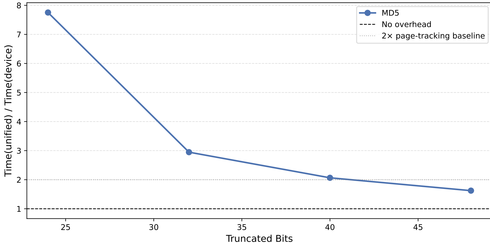
Unified Memory Overhead vs Device Memory (values > 1 = unified is slower at the same bits)
