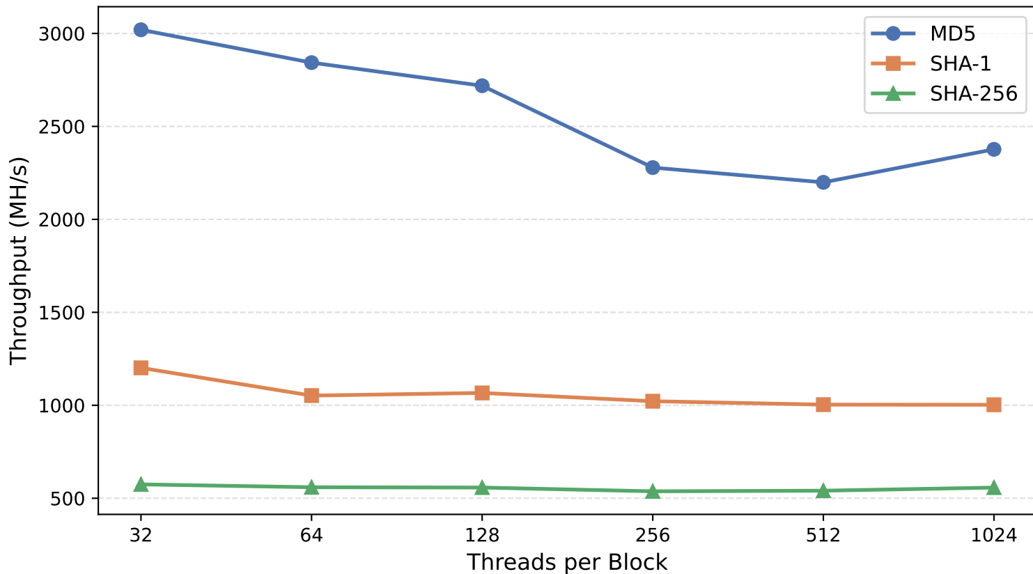
GPU Throughput vs. Threads per Block (n = 10,000,000 hashes)
