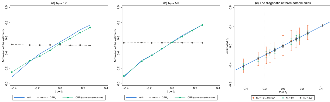
Figure 12. Monte Carlo means of CRR_{ZC} and CRR against the truth along \delta_{\beta} at 12 (a) and 50 (b) teachers, and the estimated alignment diagnostic ( \pm one Monte Carlo SD) against its true value at three sample sizes (c).
