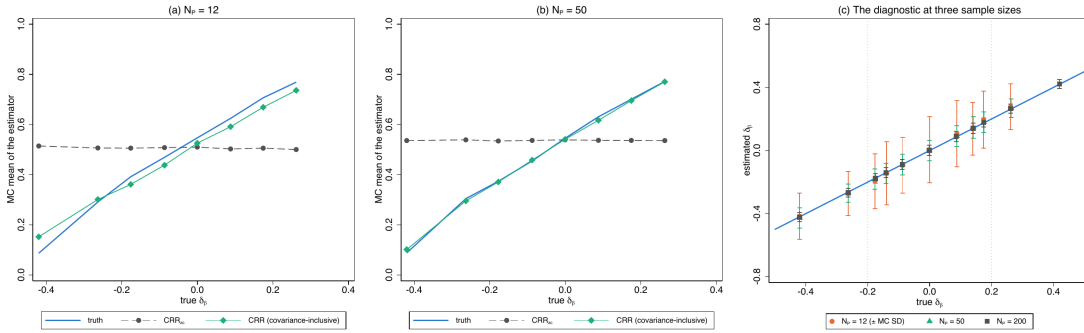
Figure 12. Monte Carlo means of CRR_{zc} and CRR against the truth along \delta_\beta at 12 (a) and 50 (b) teachers, and the estimated alignment diagnostic ( \pm one Monte Carlo SD) against its true value at three sample sizes (c).
