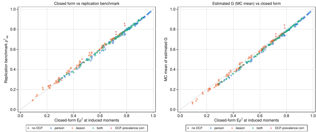
Figure 8. The DCF-extended closed forms overlaid on the simulation benchmarks across the DCF simulation's cells; deviations concentrate where the zero-covariance assumption is violated.
