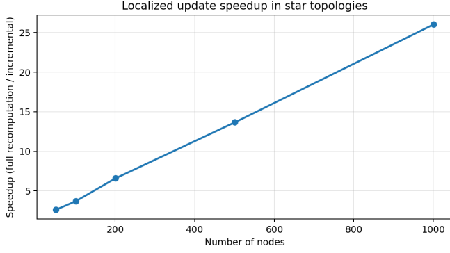
Fig. 4. Speedup for localized updates in star topologies, using full recomputation after the same update as the baseline.
