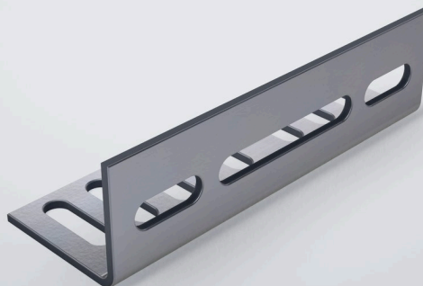
SG 60 170 Guida 60 × 170 mm
