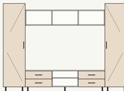
Living-room wall unit 2,800 × 2,000 width 2,200–3,600 mm
