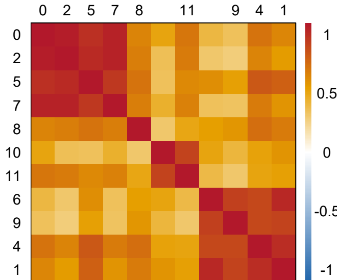
Barabasi-Albert GCM
