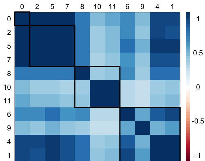
Barabasi-Albert GCM
