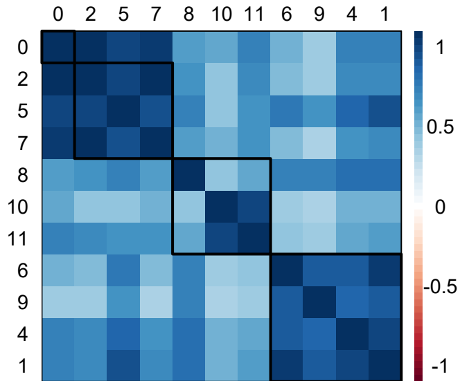
Barabasi-Albert GCM
