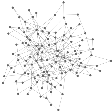
Barabasi-Albert network
